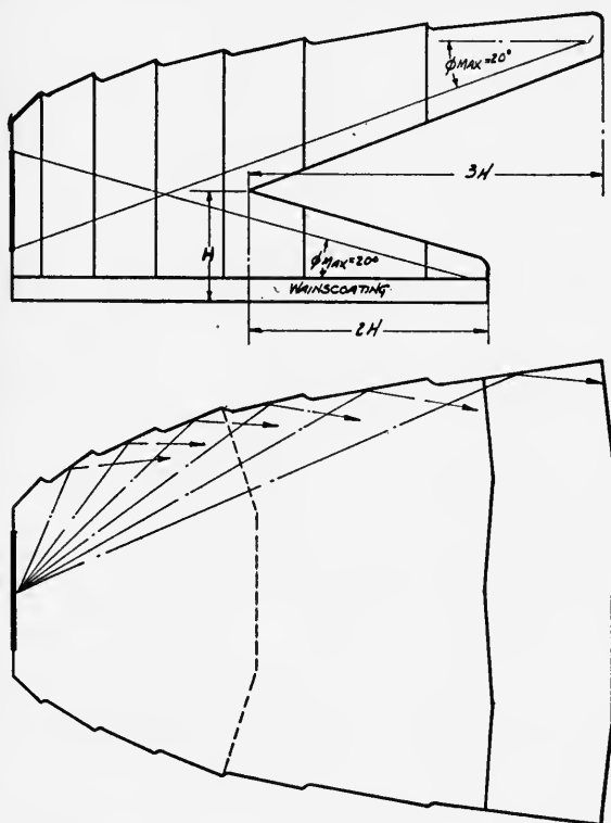
FIG. 3. Elevation and plan of theater of type discussed in the text.
